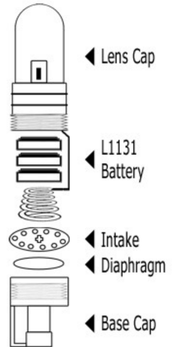
BL-31 Assembly
